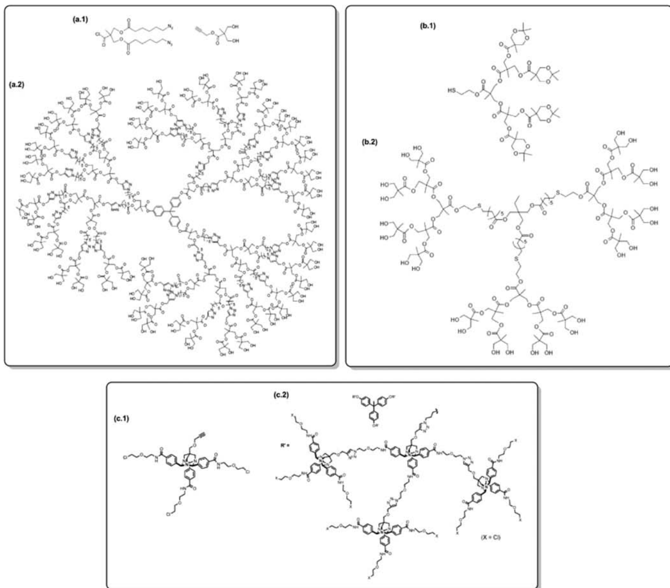
Figure 4. (a) Alternating polyester dendrimer: (a.1) AB 2 dendrons, (a.2) fourth generation (G4) dendrimer resulting from accelerated synthesis. (b) Alternating polyester dendrimer: (b.1) macrothiol-dendron bearing latent hydroxyls, (b.2) hydroxyl-terminated dendrimer based on macrothiol-dendrons. (c) Degradable TAA-based dendrimers: (c.1) degradable TAA monomer, (c.2) generation 2 (G2) of TAA-based dendrimers.
