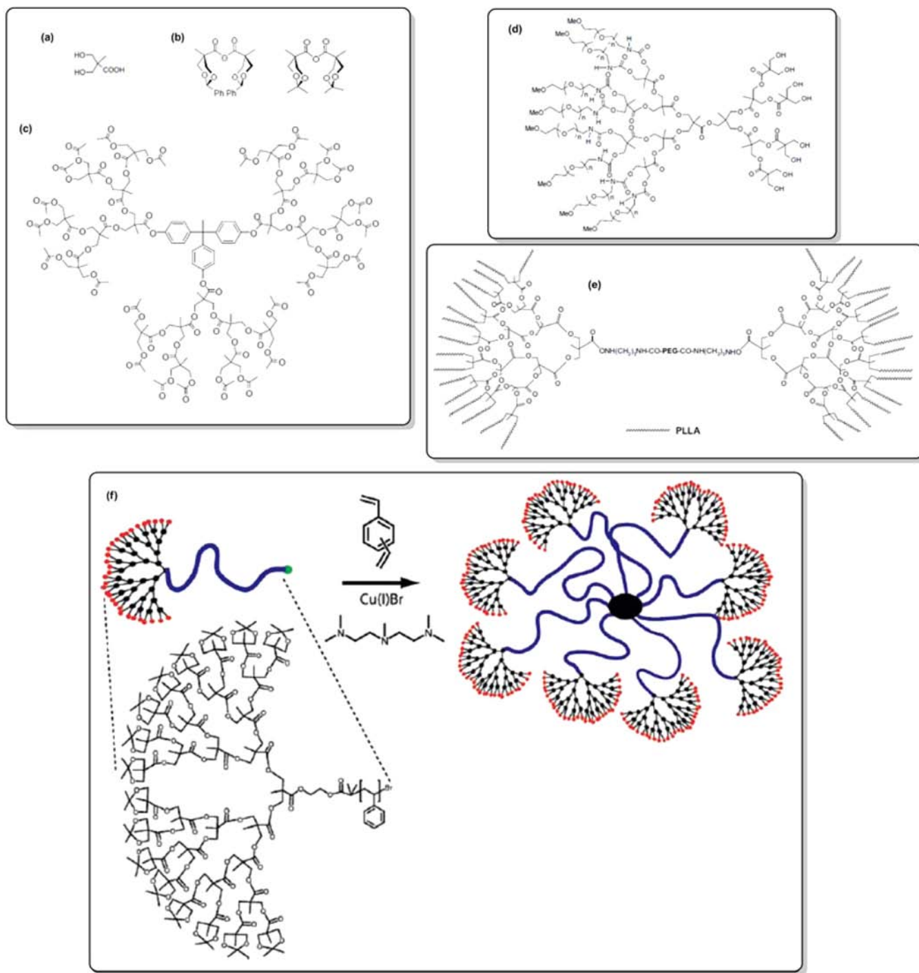
Figure 2. Bis-HMPA based dendrimers (a) 2,2-bis(hydroxymethyl)propanoic acid (bis-HMPA). (b) Protected anhydrides for the synthesis of bis-HMPA based dendrimers. (c) Generation 3 (G3) of the first synthesized bis-HMPA dendrimer. (d) "Bow-tie" dendrimer. (e) Structure of dumbbell-shaped triblock copolymer (adapted from Biodegradable comb-dendritic triblock copolymers consisting of poly(ethylene glycol) and poly(L-lactide): Synthesis, characterizations, and regulation of surface morphology and cell responses, Gong, F., Cheng, X., Wang, S., Wang, Y., Gao, Y., Cheng, S. Polymer 2009 , 50 , 2775–2785 reprinted with permission from Elsevier). (f) Synthesis of Generation 5 functionalized Core Cross-linked Star (CCS) polymers via the "arm first" approach. (Reproduced from Macromolecules 2007 , 40 , 7855–7863 with permission from The Royal Society of Chemistry).
